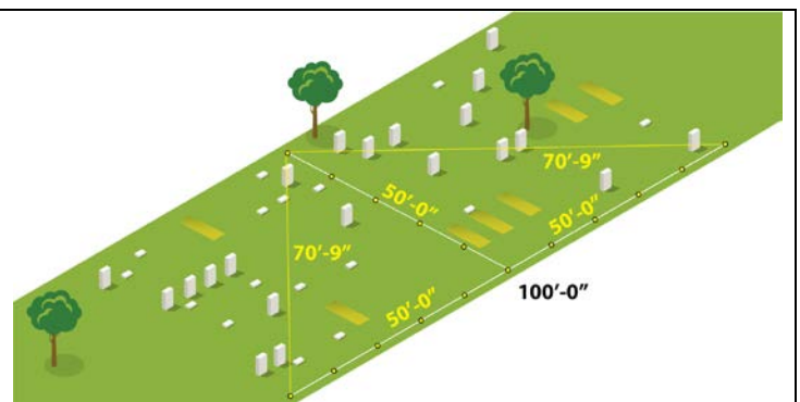
Set the perpendicular 50-foot rope
